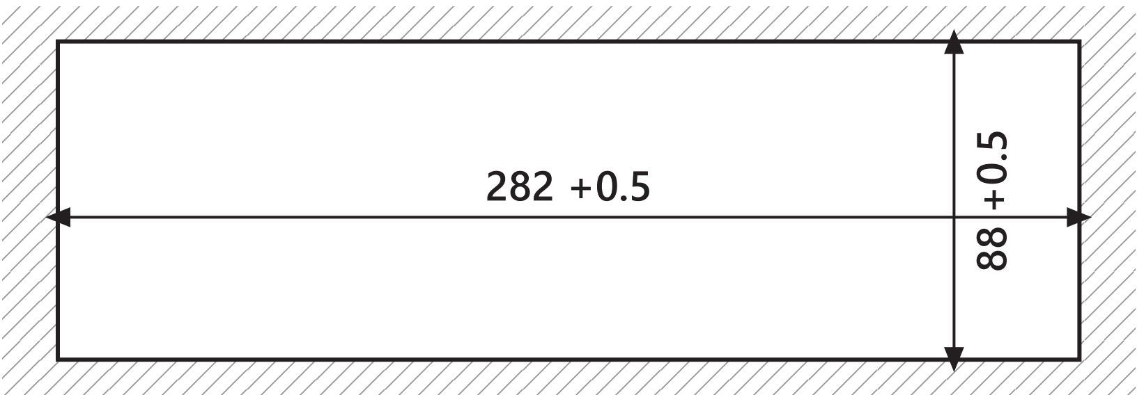
Panel cut-out
